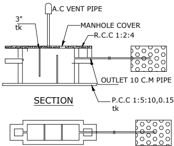
PLAN OF SEPTIC TANK & TRENCH
