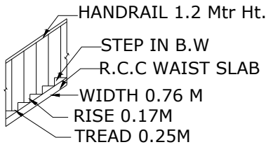
STAIR DETAIL
