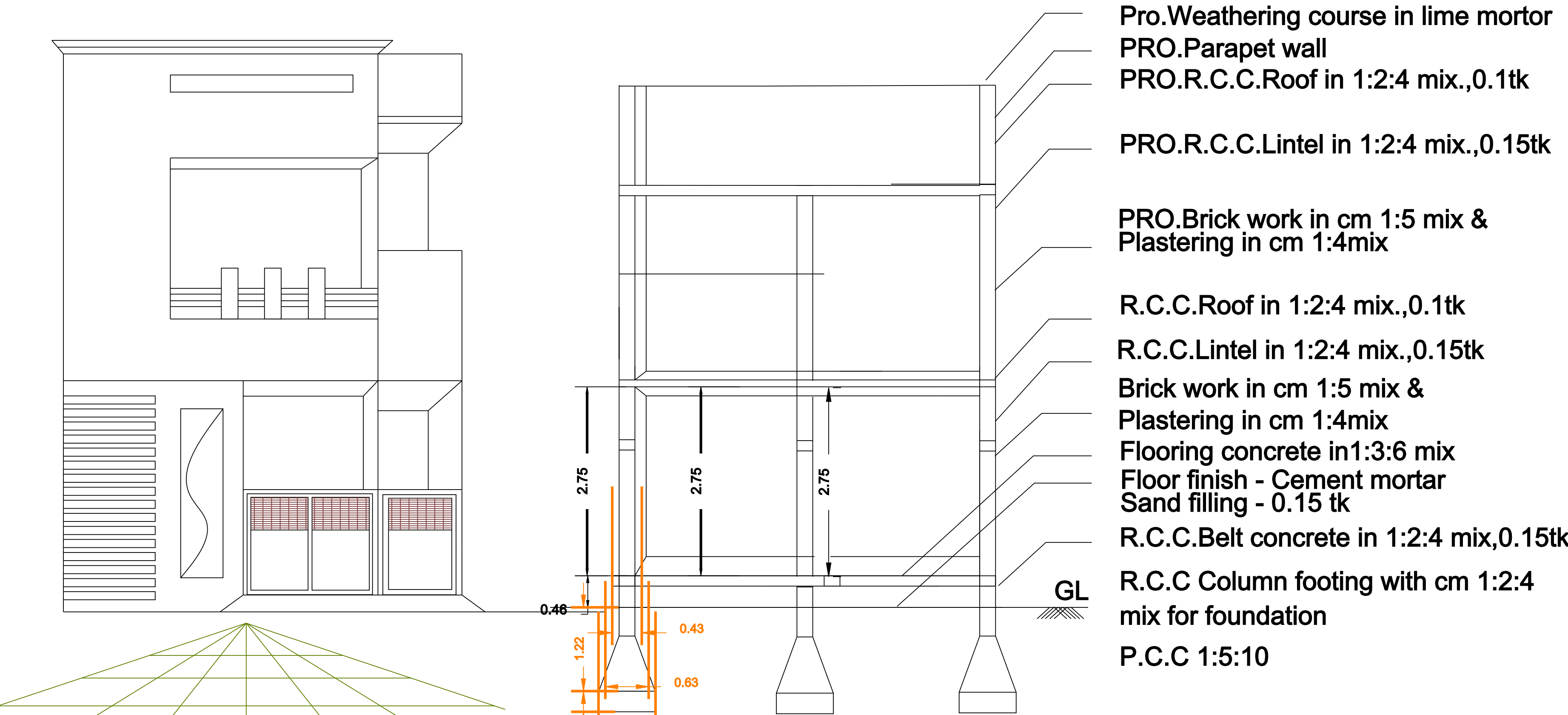
ELEVATION 5.80m SECTION ON - AB 5.80m PARVATHI AMMAL CENT AMMAL HOUSE SITE 5.80m
