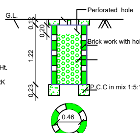
PERCOLATION PIT FOR 30 Sq. m. (Scale:- 1:50)
