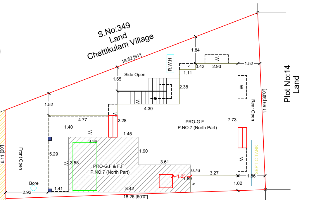
SITE PLAN Scale 1 in 100
