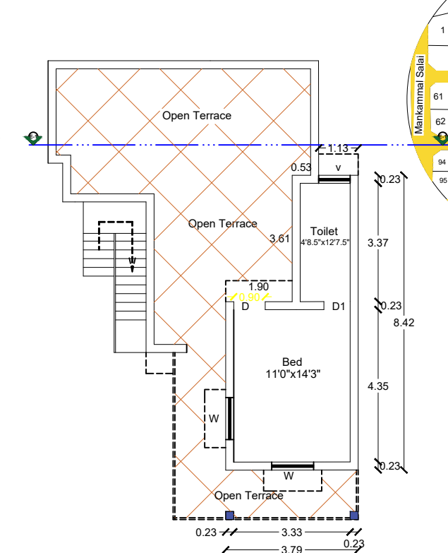
PRO-FIRST FLOOR
