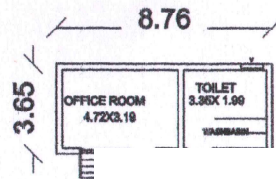
PROPOSED FLOOR P
