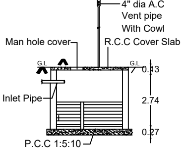
SECTION
