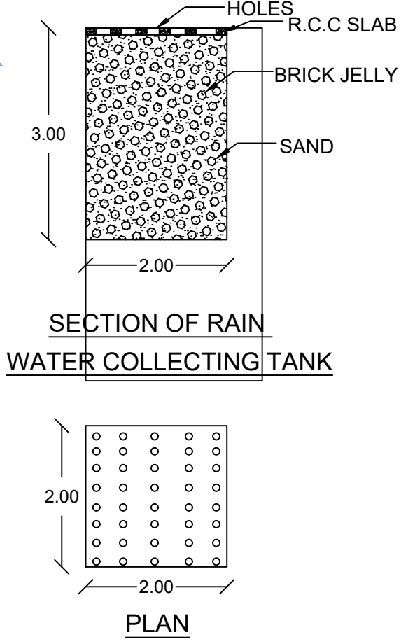
PLAN
