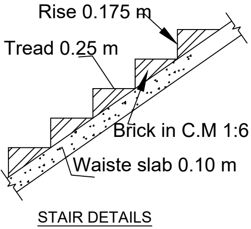
STAIR DETAILS
