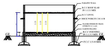
SECTION 2 - A A
