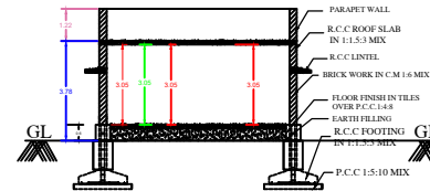
SECTION 1 - A A
