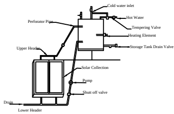
Details Of Solar Water Heater (NTS)
