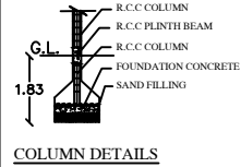
COLUMN DETAILS
