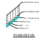
STAIR DETAIL
