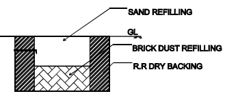
DETAILS OF RAIN WATER HARVESTING
