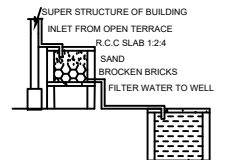
RAINWATER HARVESTING
