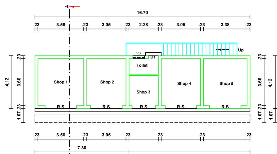
EXG.GROUND FLOOR
