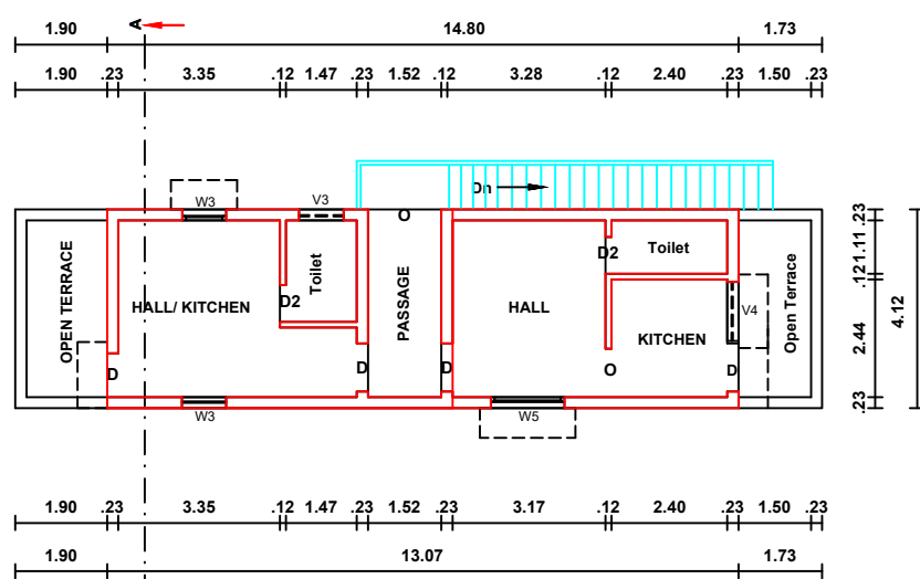
PRO. FIRST FLOOR
