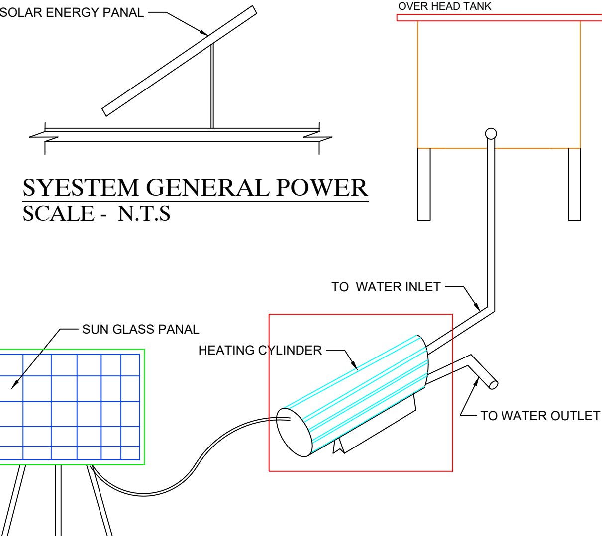
SOLAR WATER HEATING SYESTEM SCALE - N.T.S
