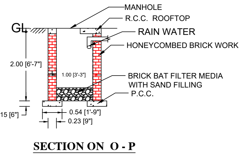
SECTION ON O - P
