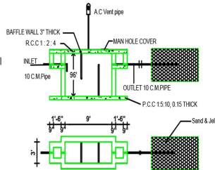
SEPTIC TANK AND TRENCH
