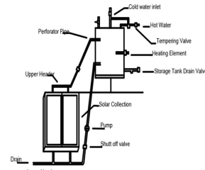
Details of solar water Heater (NTS)
