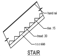
STAIR
