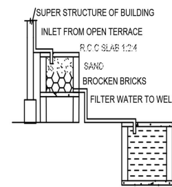
RAINWATER HARVESTING
