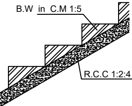
STAIRCASE
