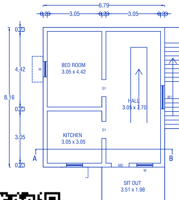
JND FLOOR PLAN
