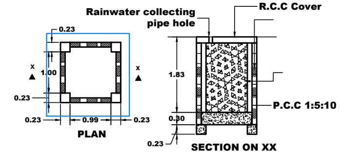
PLAN SECTION ON XX WATER_TANK_CAPACITY_L=13500LTRS
