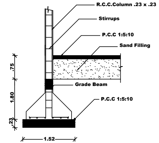
COLUMN DETAIL
