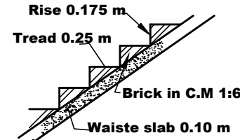
STAIR DETAILS
