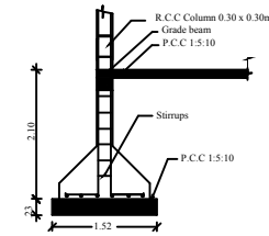
Column Detail
