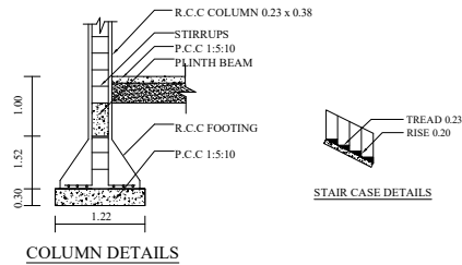
COLUMN DETAILS
