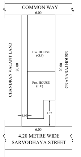
SITE PLAN SCALE 1:200
