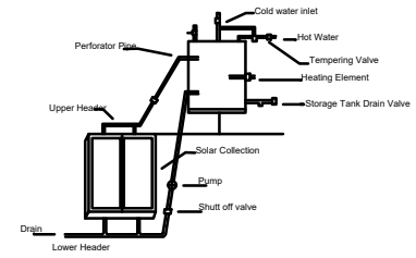
Details of solar water Heater (NTS)
