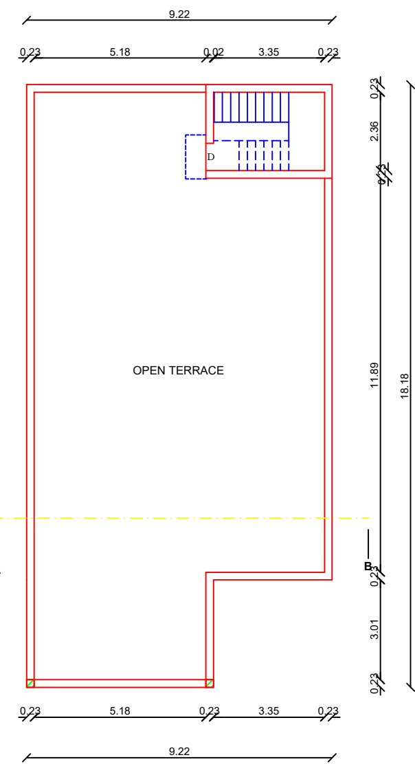
PRO. HEAD ROOM FLOOR PLAN
