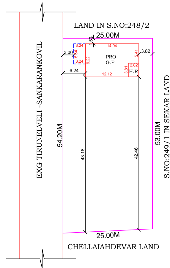
SITE PLAN (SCALE:1:400)
