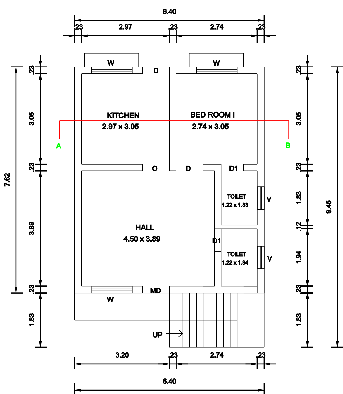
PRO GROUND FLOOR AREA
