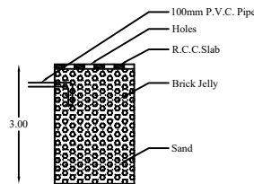
SECTION OF RAIN WATER COLLECTING TANK
