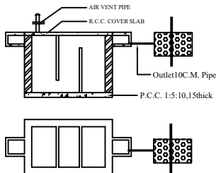
Septic Tank and Trench
