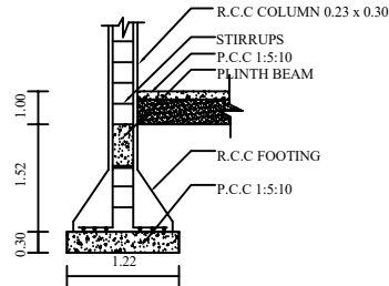
COLUMN DETAILS
