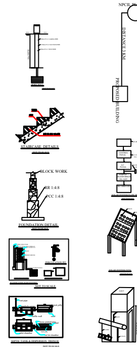
KEY PLAN NOT TO SCALE
