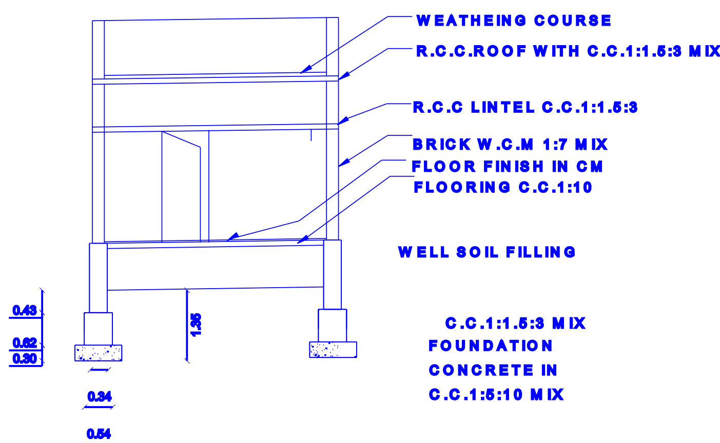
SECTION
