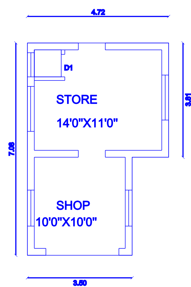
PLAN
