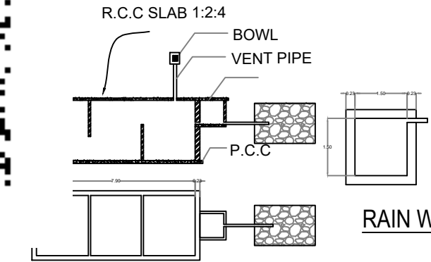
SEPTIC TANK AND TRENCH NTS
