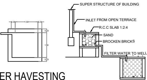
RAIN WATER HAVINGSTING
