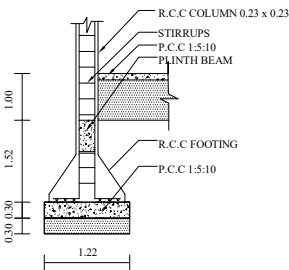
COLUMN DETAILS
