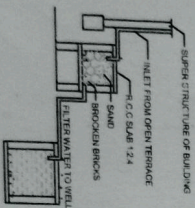
DETAILS OF FILTER BED & WELL
