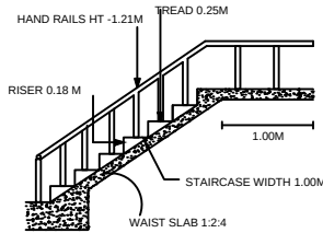
STAIRCASE DETAILS
