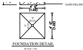
FOUNDATION DETAIL (SCALE: 1/50)
