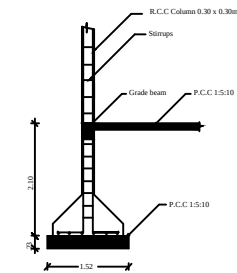
Column Detail
