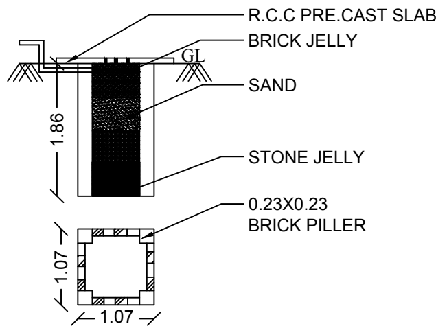
PLAN AND SECTION OF RAINWATER COLLECTION WELL
