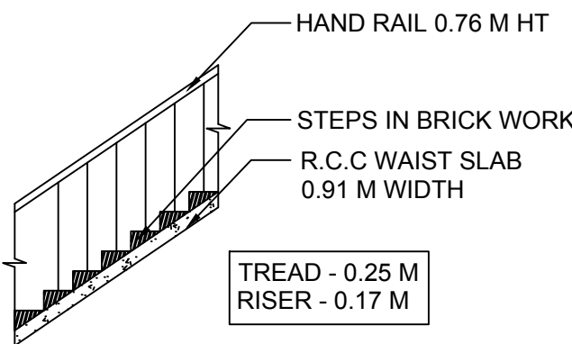
STEP DETAILS
