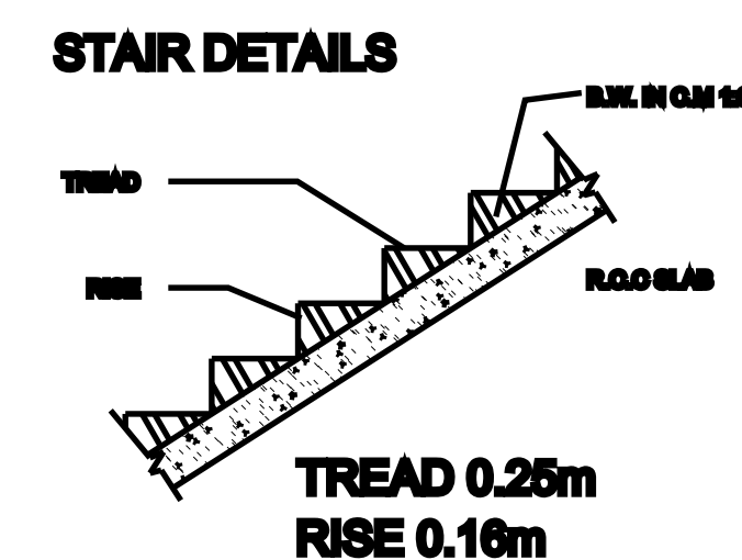
STAIR CASE
