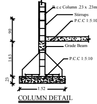
COLUMN DETAIL
