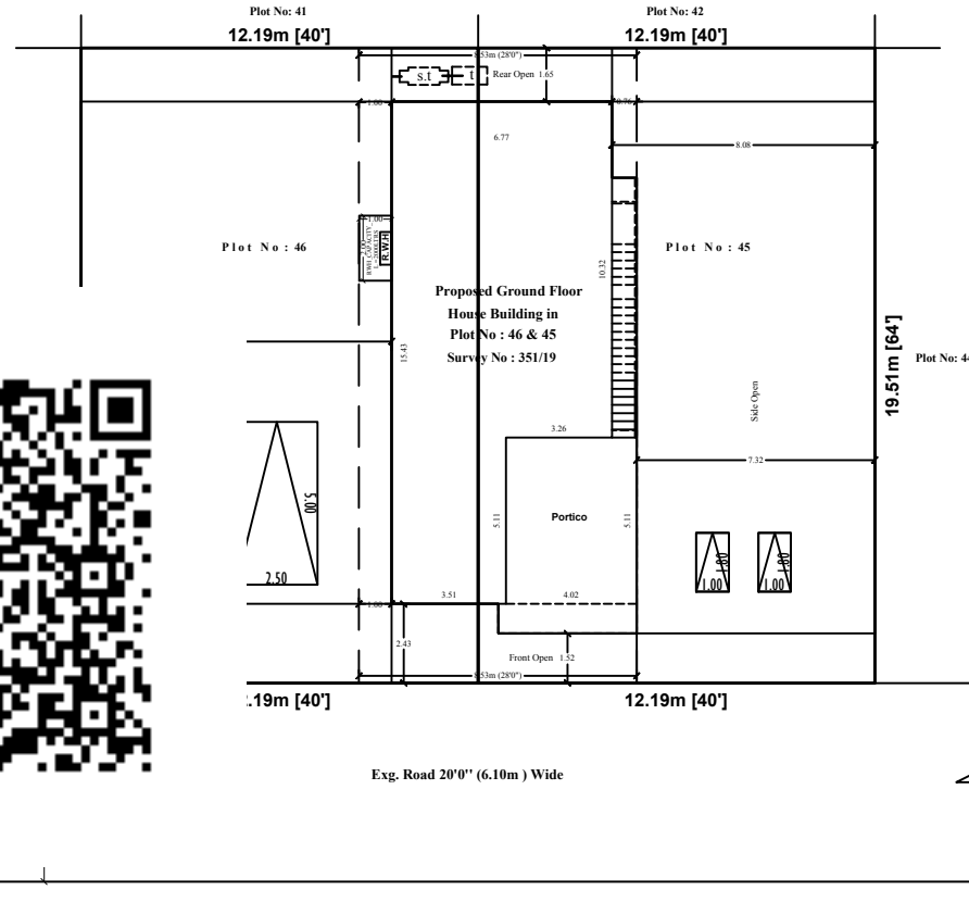
SITE PLAN
