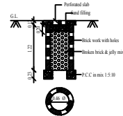
PERCOLATION PIT FOR 30 Sq. m. (Scale:- 1:50)
