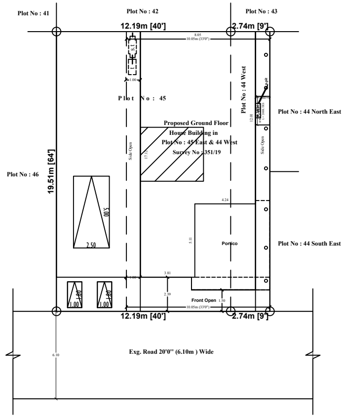
SITE PLAN
