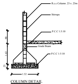
COLUMN DETAIL
