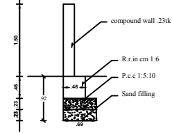
Compound Wall Detail
