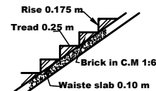
STAIR DETAILS
