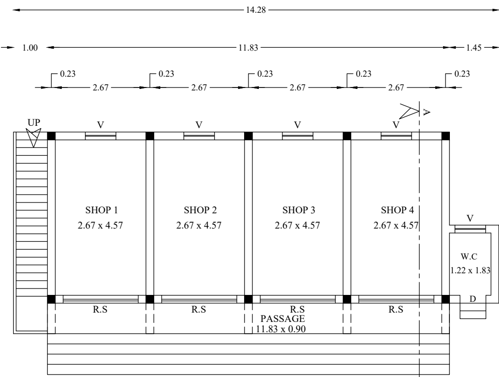
GROUND FLOOR PLAN(Approved)
