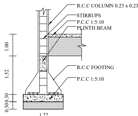
COLUMN DETAILS
