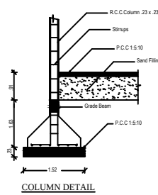
COLUMN DETAIL
