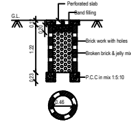
PERCOLATION PIT FOR 30 Sq. m. (Scale:- 1:50)
