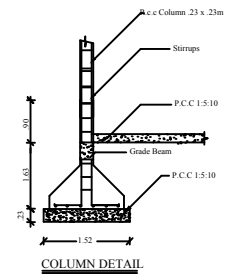
COLUMN DETAIL
