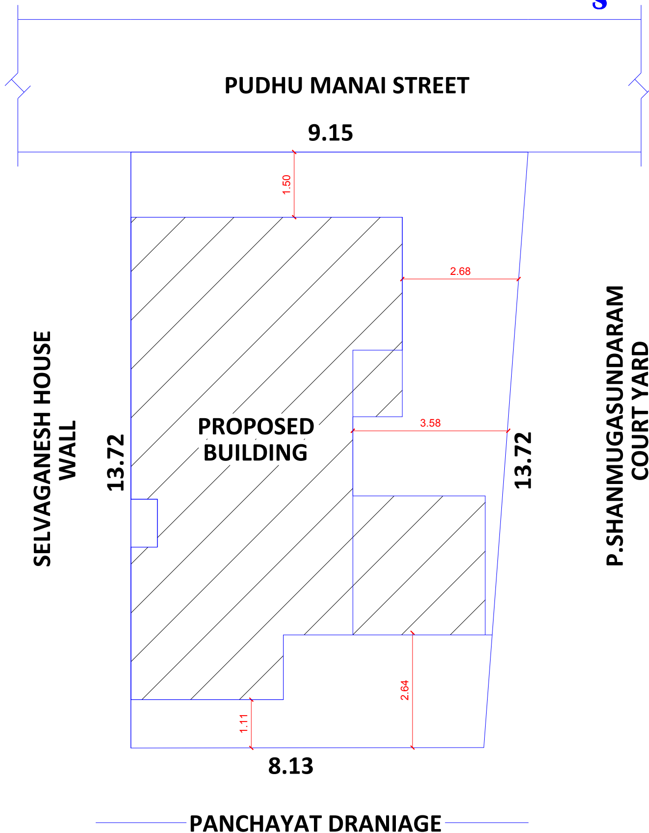
SITE PLAN
