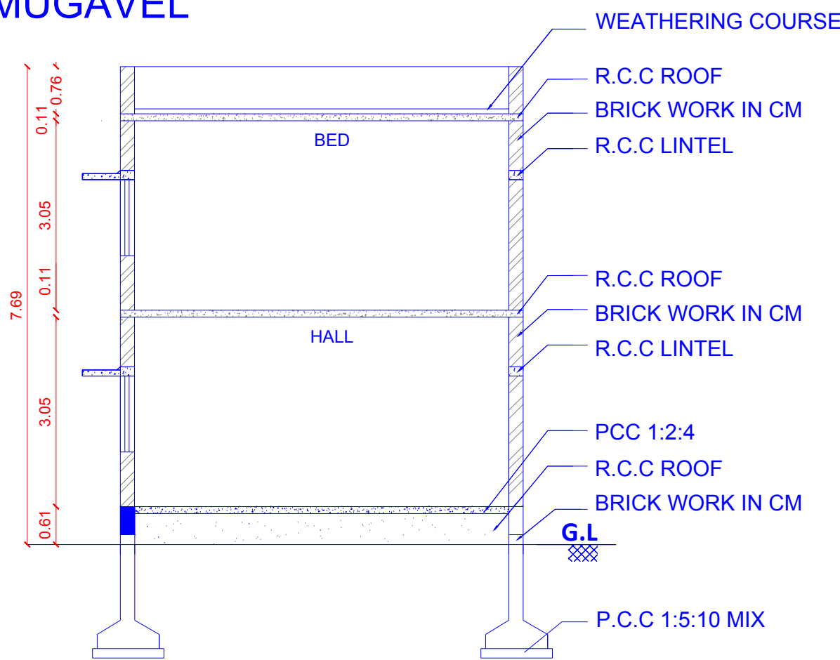
SECTION
