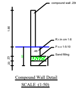
Compound Wall Detail SCALE 1:150
