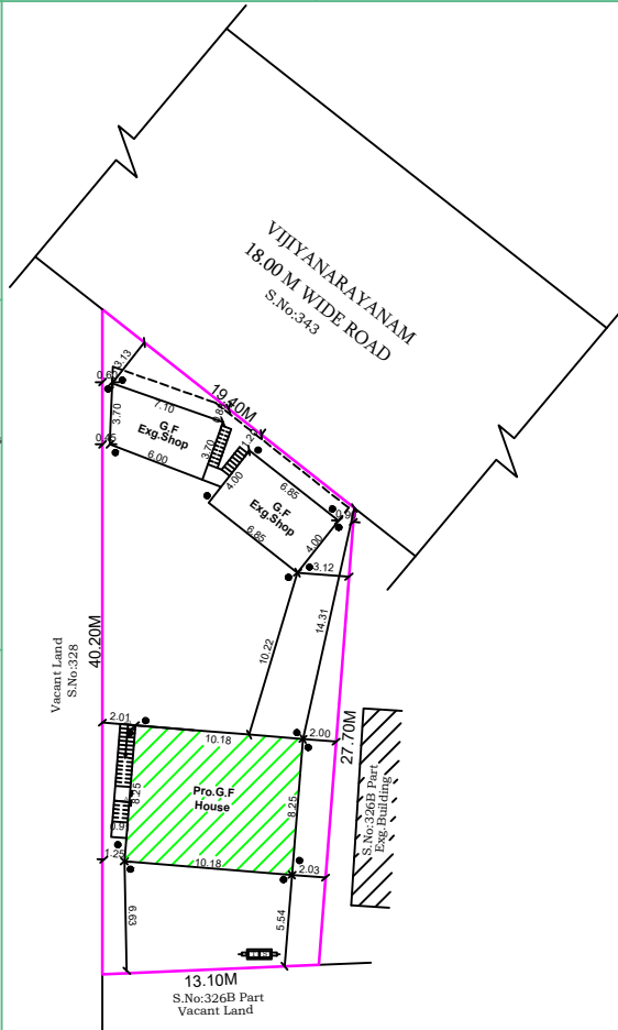
SITE PLAN
