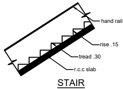
STAIR
