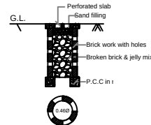
PERCOLATION PIT FOR 30' : (NOT FOR SCALE)
