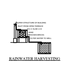
RAINWATER HARVESTING
