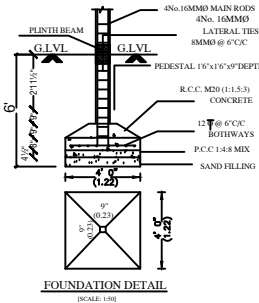
FOUNDATION DETAIL (SCALE: 1/8")
