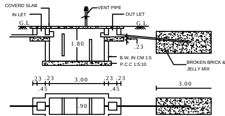
PLAN & SECTION OF SEPTIC TANK & TRENCH
