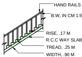
SECTION ON STAIR
