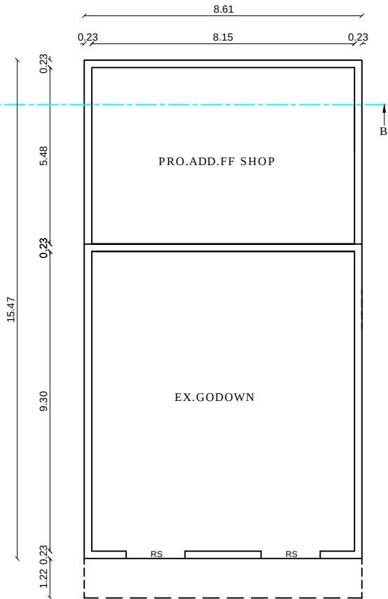
EX.FIRST FLOOR PLAN
