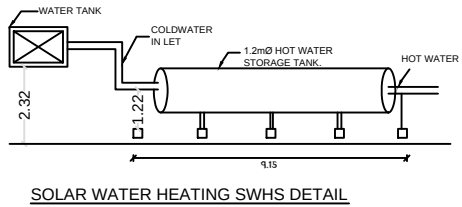
SOLAR WATER HEATING SWHS DETAIL
