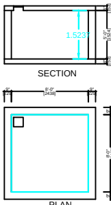
DETAILS OF COLLECTION SUMP FOR RAIN WATER HARVESTING OF ROOF TOP RAIN WATER RWV_CAPACITY_L=5000LTRS
