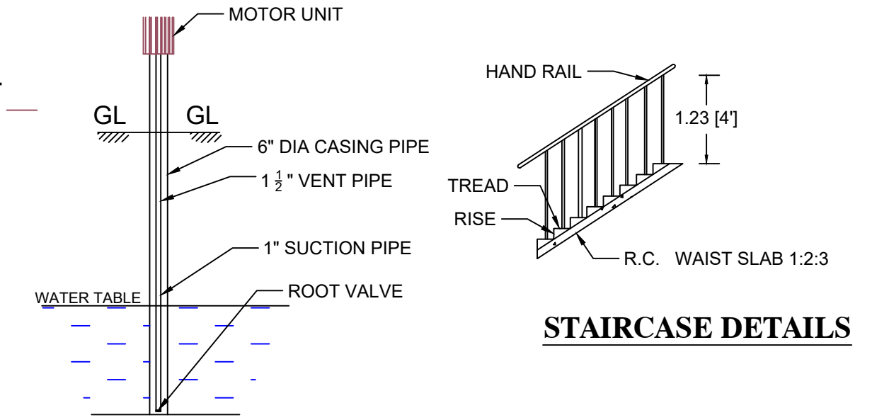
SEC.OF BOREWELL
