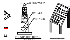
FOUNDATION DETAIL
