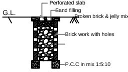
RAINWATER HARVESTING
