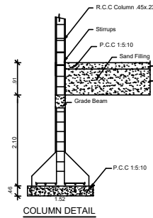
COLUMN DETAIL
