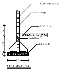
COLUMN DETAIL
