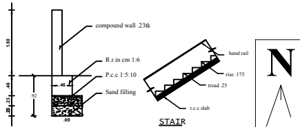
Compound Wall Detail
