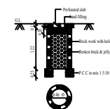
PERCOLATION PIT FOR 30 Sq. m. (Scale:- 1:50)
