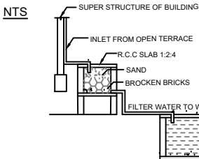
DETAILS OF FILTER BED & WELL NTS
