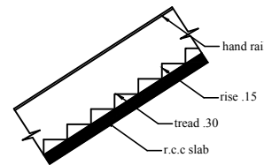
Stair
