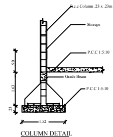
COLUMN DETAIL
