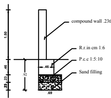
Compound Wall Detail
