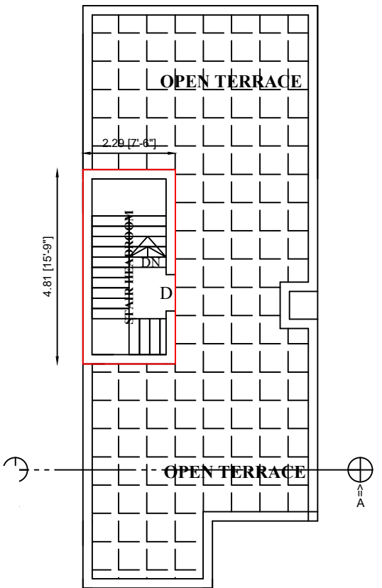
HEADROOM PLAN
