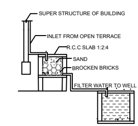
DETAILS OF FILTER BED & WELL NTS
